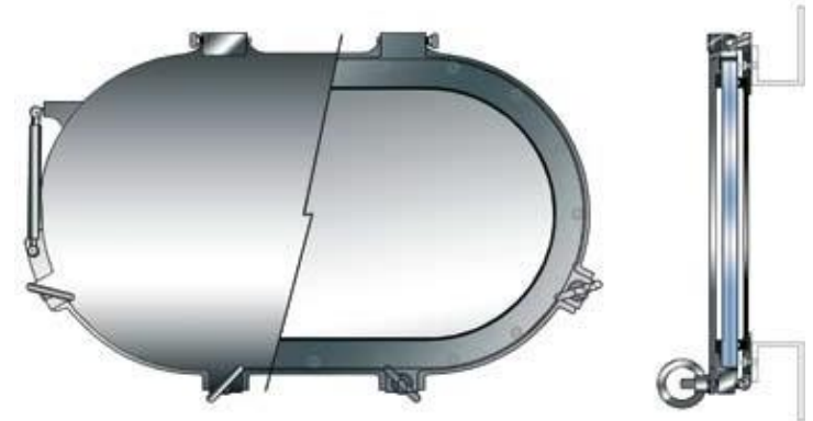
Opening Oval Portlight with Hinged Removable Deadlight
